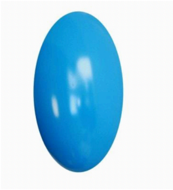
elipsoide
